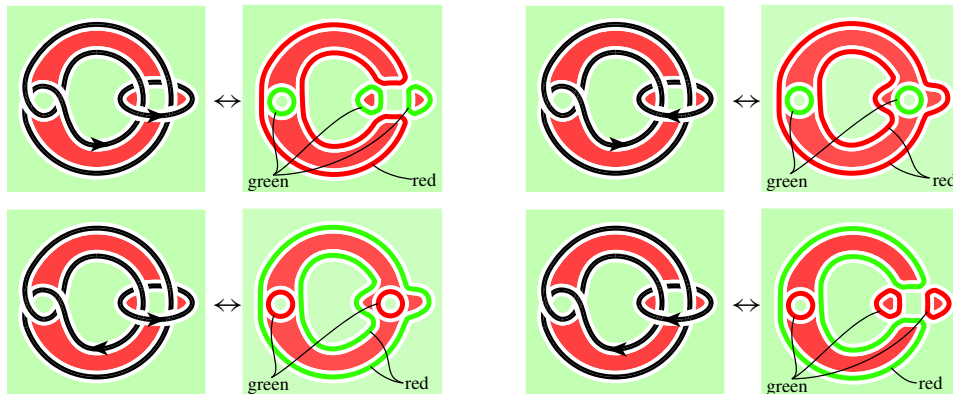
Figure 2: Generators of the Khovanov–Lee homology of the Whitehead link. (In greyscale, replace “red” and “green” with “dark” and “light”.) All four generators are in homological height zero, because the two components have linking number 0 (see Proposition 5.1 ).
