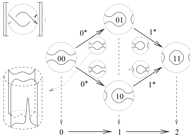
Figure 1: The Khovanov complex of a 2-crossing tangle
