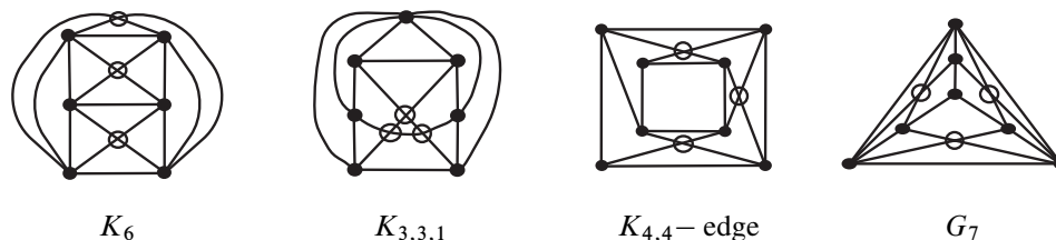
Figure 7: K_6 , K_{3,3,1} , K_{4,4} – edge and G_7 are not 3IVL.
