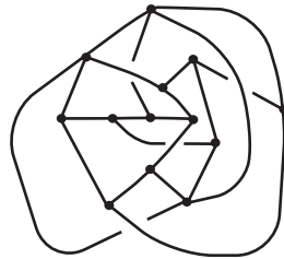
Figure 16: The graph C_{13}
