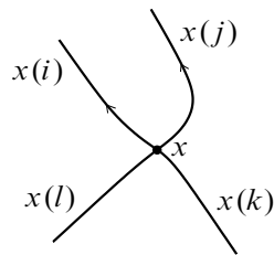
Figure 3: The labeling of edges around a crossing
