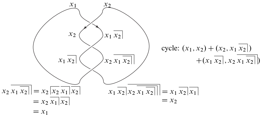
Figure 6: Cycles and knot diagrams
