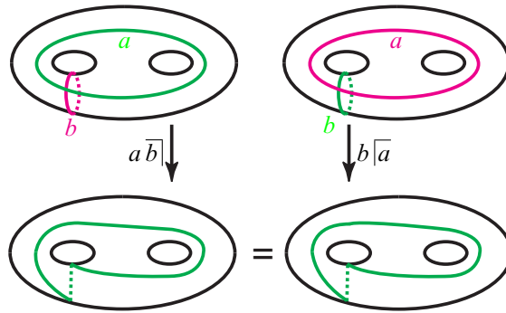
Figure 2: Fundamental relation F1
