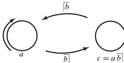
Figure 1: Conjugating twists
