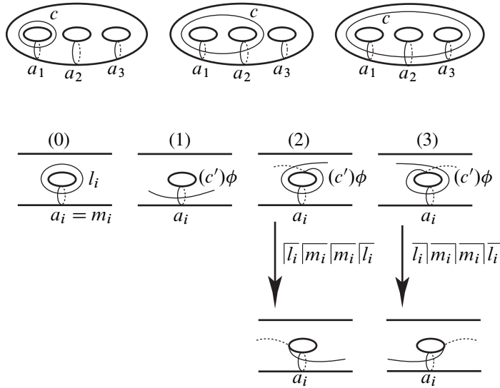
Figure 8: Standard position for tuples (c; a_1, \dots, a_t) on surface. Genus 3 example is shown.
