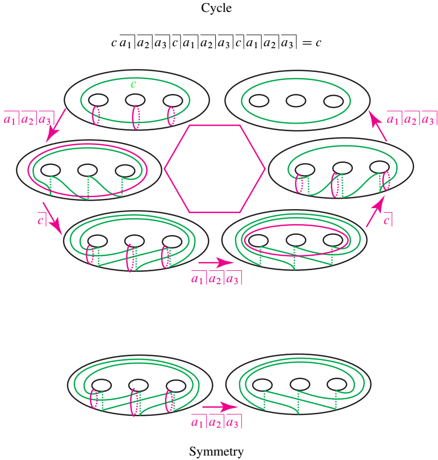
Figure 5: 2-cycle from relation (F3), and symmetry
