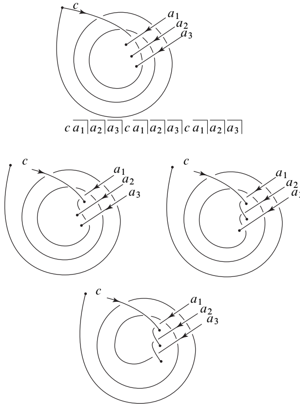
Initial moves for diagrams in the proof of the relation
