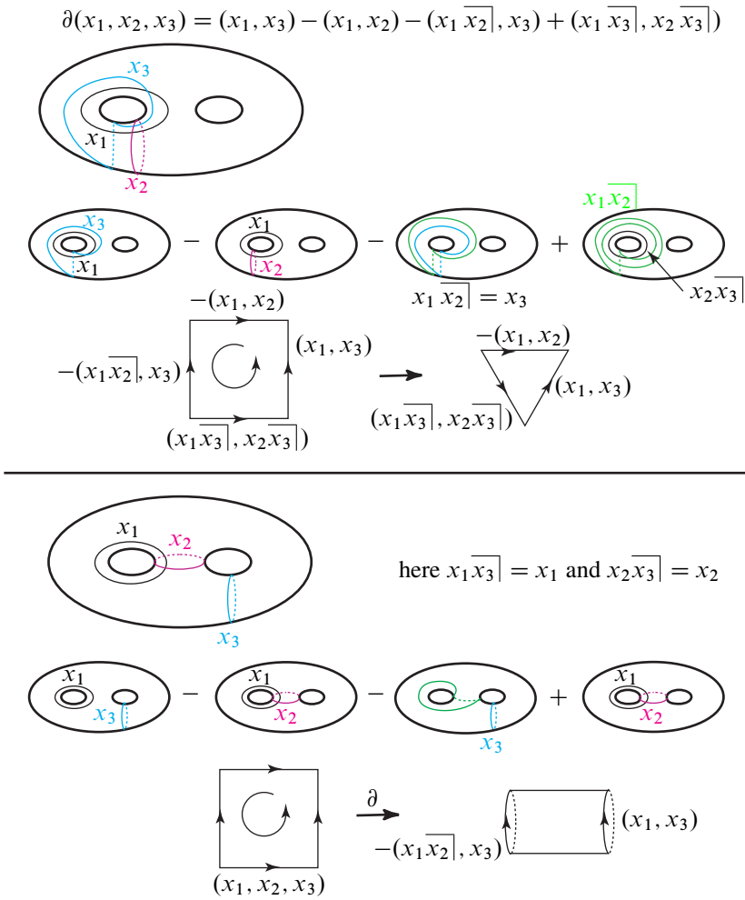
Figure 3: Boundaries of 3-simplices with identifications
