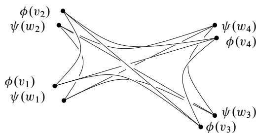
Figure 1: Points in X
