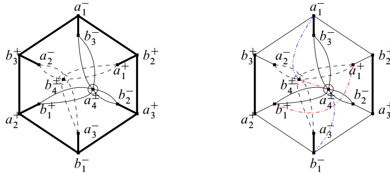
Figure 7: Lk(X, v) and Lk(X_2, v) . The circles indicate suspension points as in Figure 1. Poison Corners are indicated by bold edges. Note that although the one dot-dash edges and the two dot-dash edges appear to meet at the suspension points, they do not. A careful check shows that there are no circuits of length less than four.
