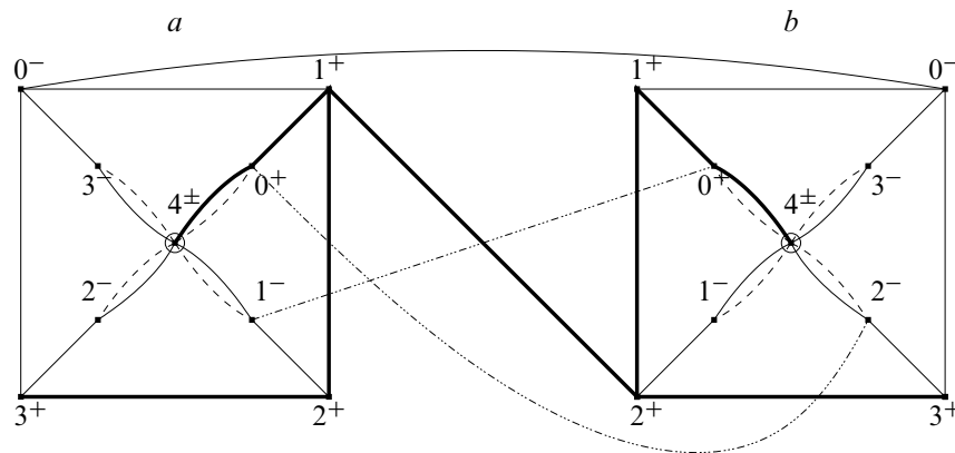
Figure 2: Lk(v, X_1) . The descending link is shown in bold.
