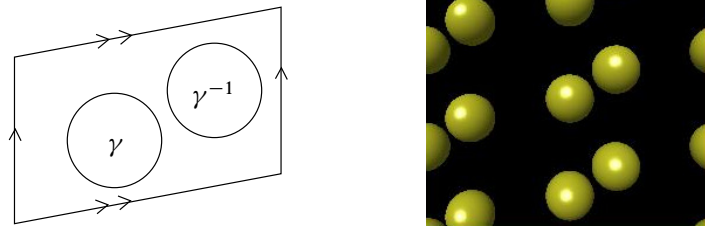
Figure 2: Left: Schematic picture of a simple Ford domain. Right: Three dimensional view of \mathcal{F} in \mathbb{H}^3 .
