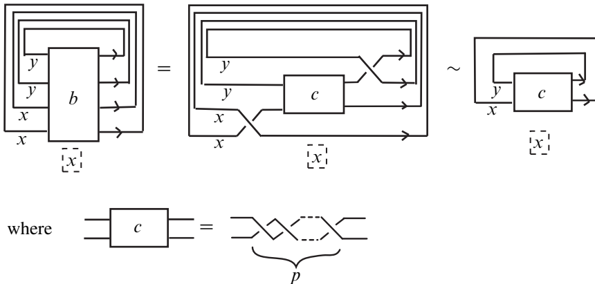
Figure 25: The shadow coloring for \widehat{b} with the base color x
