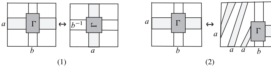
Figure 3: Equivalent moves of m -charts
