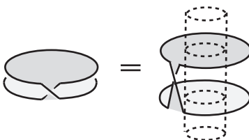
Figure 13: The disk bounded by \hat{\alpha}
