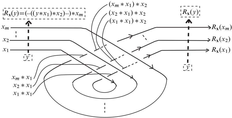
Figure 19: The braid \Delta^2
