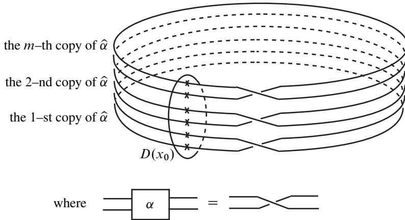
Figure 9: The closure \hat{a} of a
