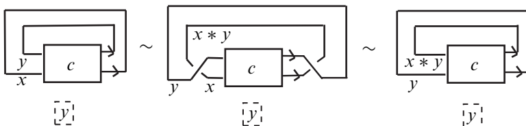
Figure 26: The shadow coloring for \widehat{b} with the base color y
