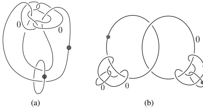
Figure 4: The manifold A
