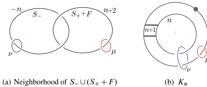
Figure 31: \mathbb{F}_n
