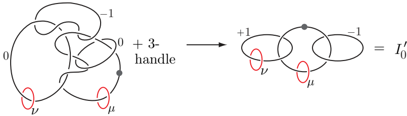
Figure 22: I'_0
