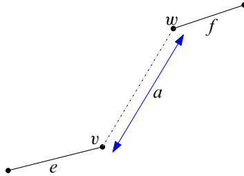
Figure 18: The situation in Case 1
