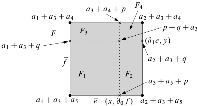
Figure 28: The graph of d in Case 2(iii). Here, p = (a_1 + a_2 + \ell(e))/2 and q = (a_4 + a_5 + \ell(f))/2 .
