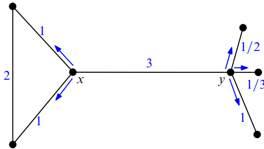
Figure 1: Computing the positive indices \text{ind}_+(x, y) , \text{ind}_+(y, x)
