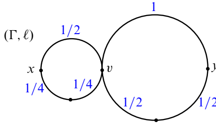
Figure 6: The graph structure on \Gamma = S^1 \vee S^1
