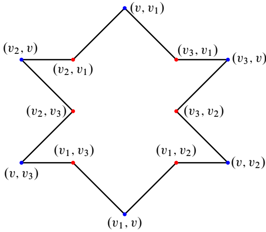
Figure 5: G_r for 0 < r \leq 1/2
