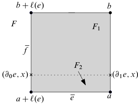
Figure 22: The separating line \bar{e} \times \{x\}
