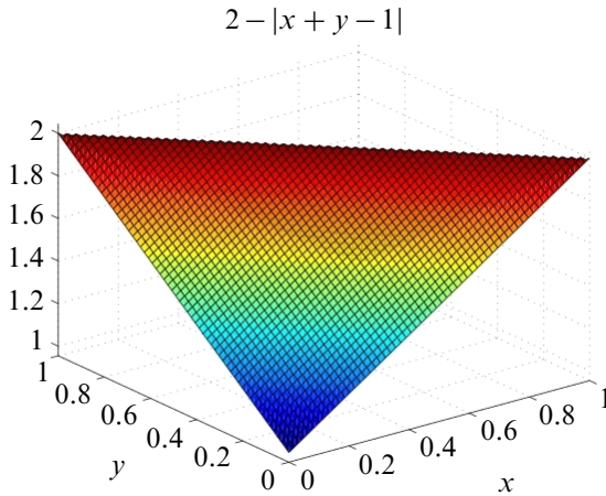
Figure 26: The graph of d \circ \chi_F with a = b = 1 and \ell(e) = \ell(f) = 1 ; it is symmetric about y = 1 - x .
