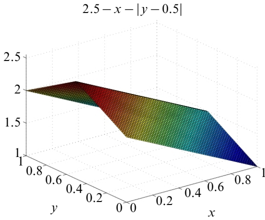
Figure 23: The graph of d \circ \chi_F with a = b = 1 and \ell(e) = \ell(f) = 1
