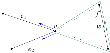
Figure 31: The situation in Case 2
