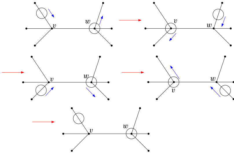
Figure 34: Generators of H_1(K_{p,q}) interpreted as cycles in H_1(F_b)
