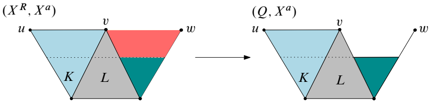
Figure 14: Deformation retraction of (X^R, X^a) onto (Q, X^a)
