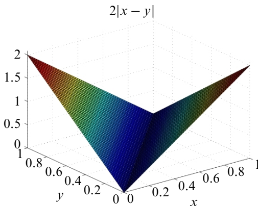
Figure 17: The metric d on a diagonal 2-cell F = \bar{e} \times \bar{e} with \ell(e) = 2
