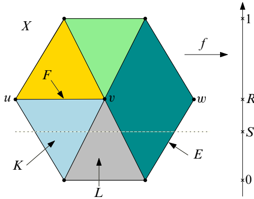
Figure 8: The hexagon X
