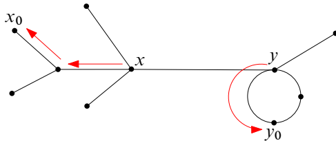
Figure 2: Finding an index zero configuration (x_0, y_0)
