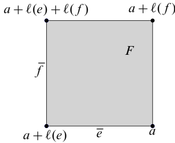
Figure 19: d \circ \chi_F extends to an affine map \mathbb{R}^2 \rightarrow \mathbb{R}
