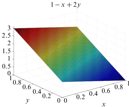
Figure 20: The graph of d \circ \chi_F with a = 0 , \ell(e) = 1 and \ell(f) = 2
