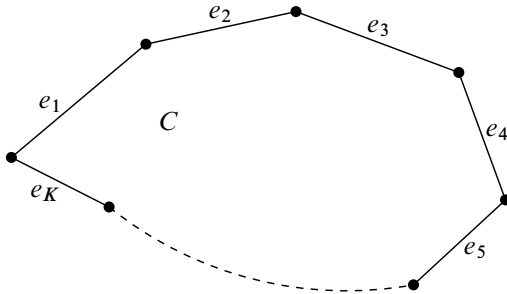
Figure 15: A cycle C = (e_1, \dots, e_K) in a simple graph
