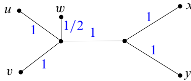
Figure 4: The labelled tree T
