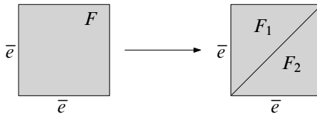
Figure 16: Subdividing a diagonal 2-cell F = \bar{e} \times \bar{e}
