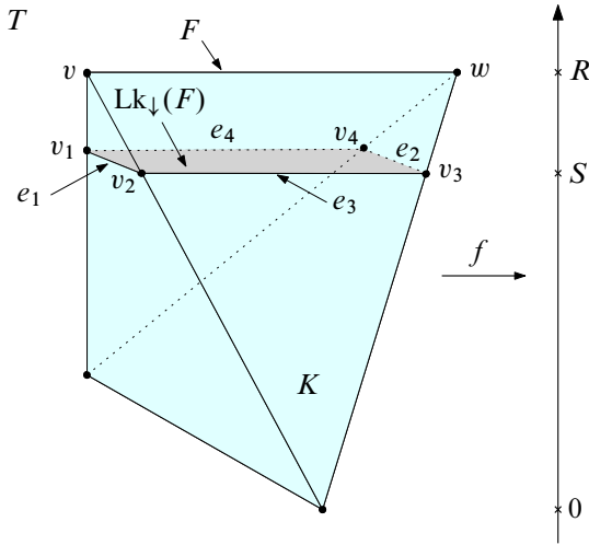
Figure 10: The solid tetrahedron T
