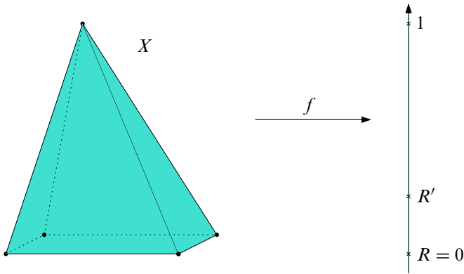
Figure 11: The pyramid X and the affine Morse–Bott function f
