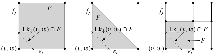
Figure 30: g -Descending cells F incident to (v, w) , with \text{Lk}_\downarrow(v, w) \cap F shown in each case
