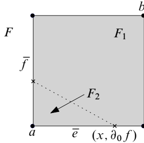
Figure 25: The separating line on which d is constant
