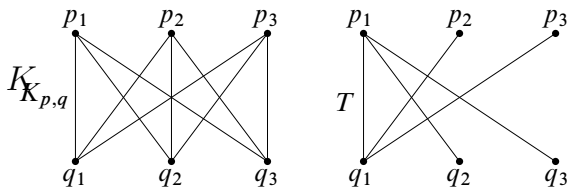
Figure 33: The descending link \text{Lk}_\downarrow(v, w) = K_{p,q} and the maximal tree T
