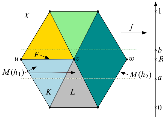
Figure 13: The mapping cylinders M(h_1) and M(h_2)
