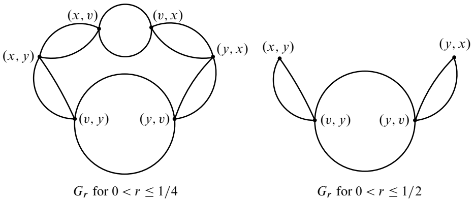
Figure 7: The graphs G_r
