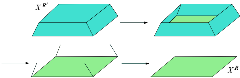
Figure 12: The steps of the deformation retraction from Proposition 3.19
