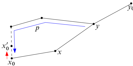
Figure 3: The point x'_0 and the arc p
