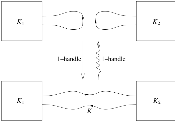
Figure 1. In this figure we show how the connect sum K = K_1 \# K_2 of two knots K_1, K_2 is obtained from the disjoint union of the knots by a knot cobordism consisting of a single 1–handle attachment (the straight arrow), and likewise the reverse direction (the bendy arrow).
