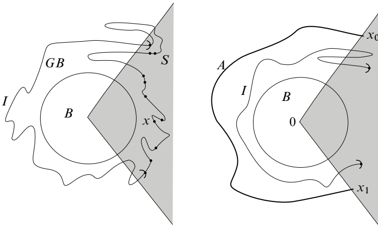
(a) I \subset (\partial(GB) \setminus \overline{Gx}) is a spanning interval. Dots indicate points in the orbit of x .
