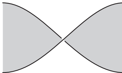
Figure 4: Colouring convention for alternating diagrams
