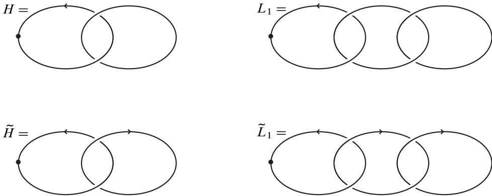
Figure 2: Two partly oriented links H and L_1 and two marked oriented links \tilde{H} and \tilde{L}_1
