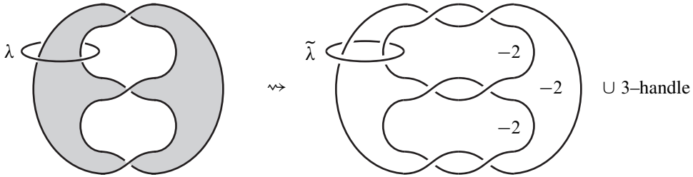
Figure 5: A link diagram and the double cover of D^4 branched along the black surface, showing the preimage of a curve \lambda .
