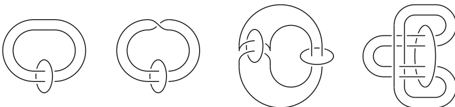
Figure 1: Some links bounding \chi = 1 surfaces in the four-ball: the connected sum of two Hopf links, the (2, 4) -torus link, the Borromean rings and the connected sum of Hopf and Whitehead links.
