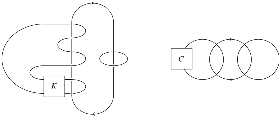
Figure 3: Partly oriented links L_2 \# H and L_3 \# H . The band shown passing through the box marked K is tied in the knot K with zero framing; see Cha, Kim, Ruberman and Strle [6].
