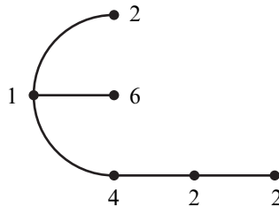
Figure 6: The plumbing diagram for the Montesinos link L_4
