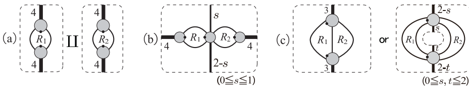
Figure 1: Possible positions of two digons R_1 and R_2
