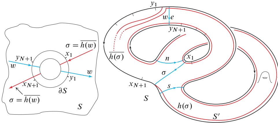
Figure 9: Two views of \partial S
