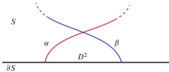
Figure 5: A boundary trivial intersection
