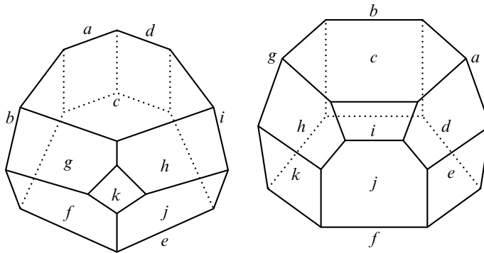
Figure 2: Indices of facets of \mathcal{P} and \mathcal{Q}
