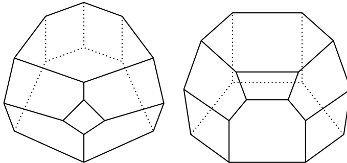
Figure 1: \mathcal{P} and \mathcal{Q}
