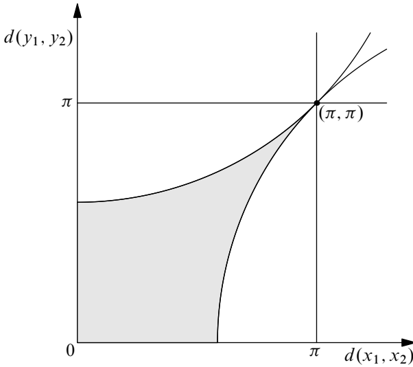
Figure 1: (x_1, y_1) and (x_2, y_2) are in the same fiber of f only if (d(x_1, x_2), d(y_1, y_2)) is in the shaded region.
