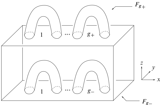
Figure 2.2: The cube C_{g_-}^{g_+} with g_- tunnels and g_+ handles
