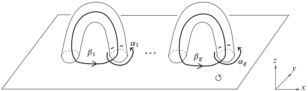
Figure 2.1: The model surface F_g of genus g \geq 0 , together with its system of meridians and parallels (\alpha, \beta)
