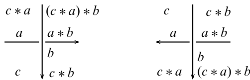
Figure 11: Shadow coloring at a crossing
