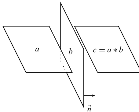
Figure 5: Coloring rules at a double curve
