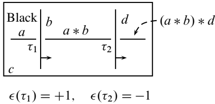
Figure 10: Adjacent triple points with different signs
