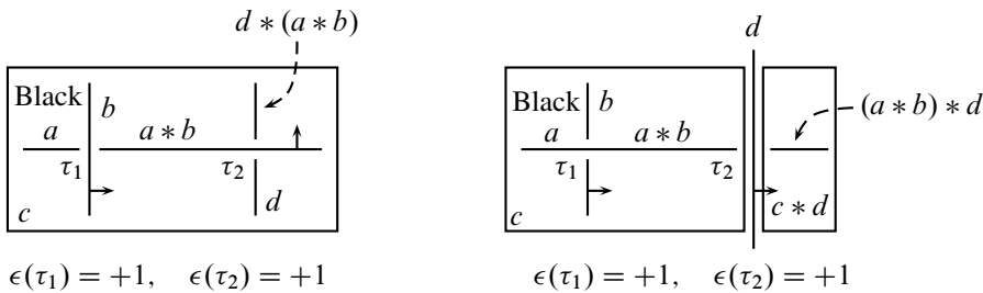
Figure 9: Two possibilities of adjacent triple points with the same sign
