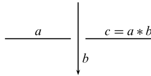
Figure 1: The proper coloring rule
