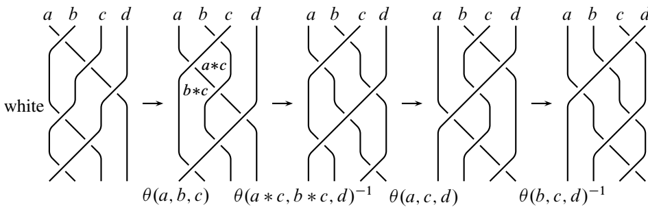
Figure 7: Left-hand side of the tetrahedral move
