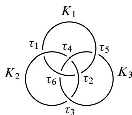
Figure 13: The Borromean rings
