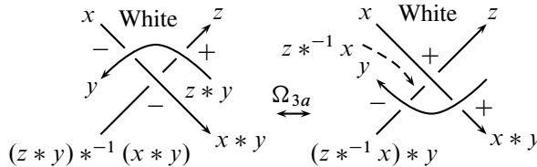
Figure 4: Proper colorings under \Omega_{3a}
