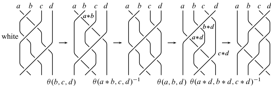
Figure 8: Right-hand side of the tetrahedral move
