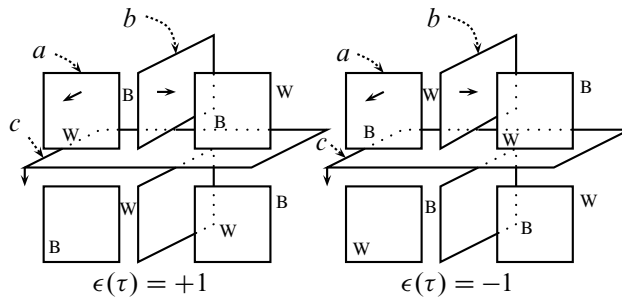
Figure 6: Signs of triple points
