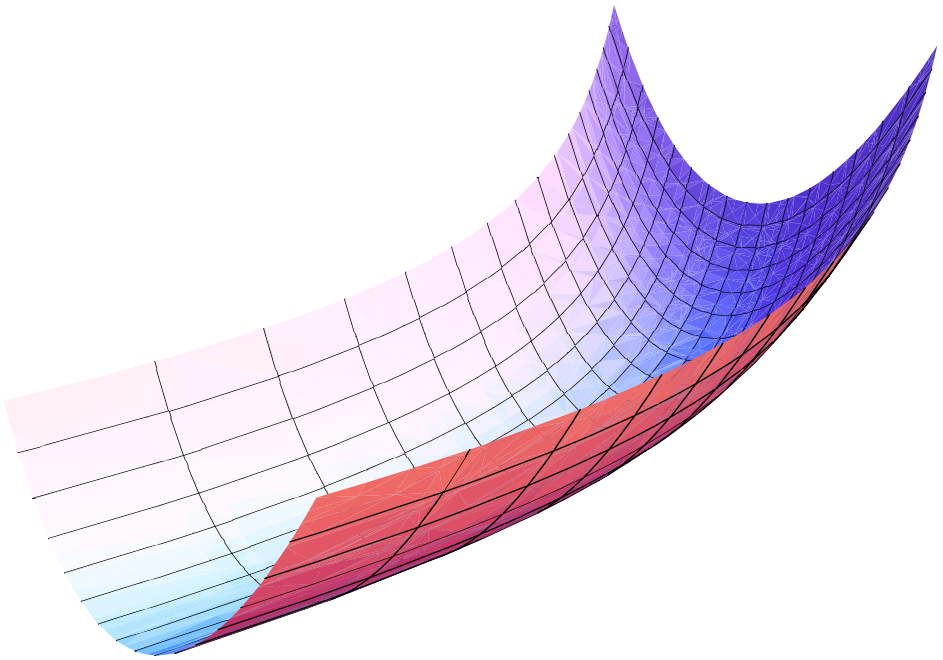
Figure 1: A generic orbit of H
