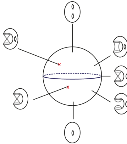
Figure 1: Example of a bLf with one circle of folds and two Lefschetz points.
