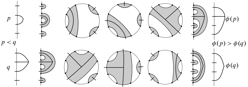
Figure 5: The order-reversing automorphism \phi of \text{NC}_n (when read from left to right), or its inverse \phi' (when read from right to left)
