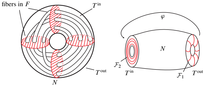
Figure 1: Constructing a Hirsch foliation
