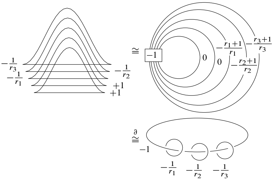
Figure 1: Contact structures on M(-1; r_1, r_2, r_3) , followed by the smoothed surgery diagram of the underlying 3-manifold and its standard presentation; when referring to them as 4-manifolds, we assume inverse slam-dunks to be done.
