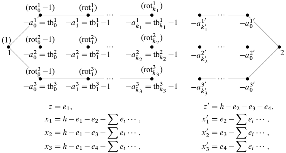
Figure 3: Plumbing graph \Gamma (left) and its dual \Gamma' (right) with denoted self-intersections and evaluations of characteristic covector c , (\cdot) = \langle c, v \rangle , on the manifold side; the central and the first vertices on legs are given in generating classes of H_2(R; \mathbb{Z}) .
