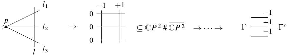
Figure 2: Construction of the 4-manifold R = \mathbb{C}P^2 \# n\overline{\mathbb{C}P^2} ; at the end, the two plumbings are glued together along the exceptional spheres from the last blow-up of each singular fiber, and (not shown) all regular fibers.
