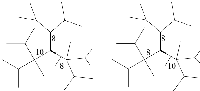
Figure 10: Cloud representations for [c_4] (left) and [d_4] (right) corresponding to the cells \Phi and \Psi in UD^{27}(\Gamma)
