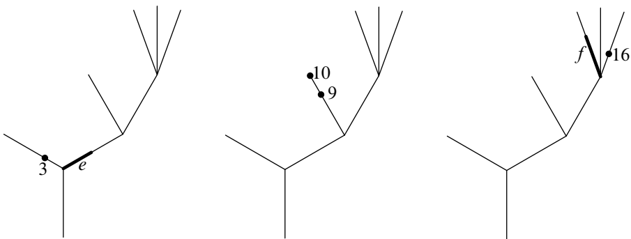
Figure 3: Three different cells in UD^2(\Gamma)
