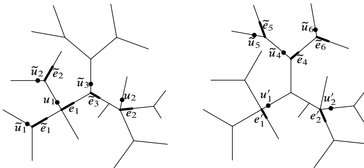
Figure 11: The critical cells \Phi and \Psi in UD^{10}(\Gamma)
