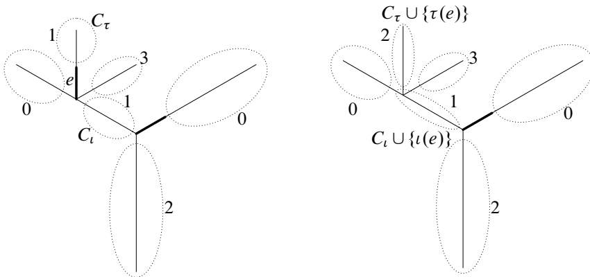
Figure 6: The cloud diagram \mathcal{C} for a standard cocycle \phi_{[c]} (left) and the cloud diagram for the cochain \mathcal{R}_{C,v} (right)
