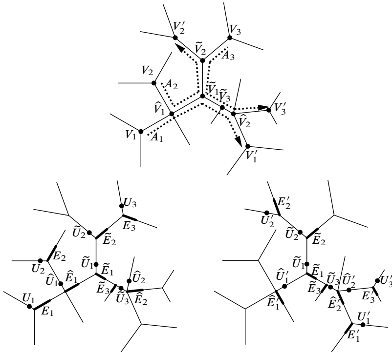
Figure 12: The critical cells \Phi and \Psi in UD^{16}(\Gamma) (bottom left and right)
