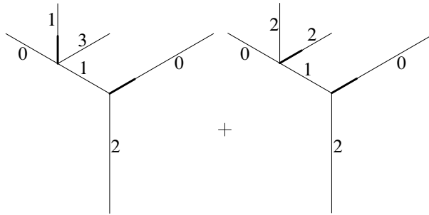
Figure 7: The sum \sum_{i=1}^{d(v)-1} \Theta_{C,v,\tau,i} with C as in Figure 6
