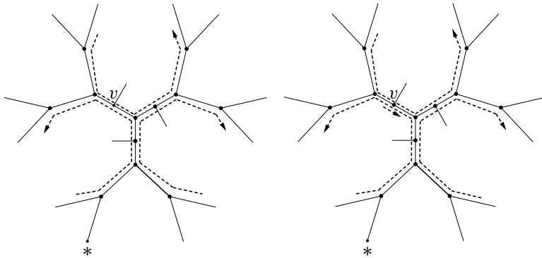
Figure 2: Two collections of arcs in a graph \Gamma
