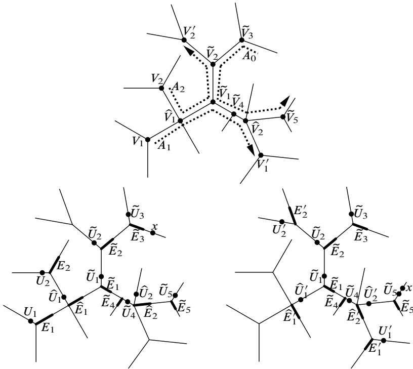
Figure 13: The critical cells \Phi and \Psi in UD^{19}(\Gamma) (bottom left and right)
