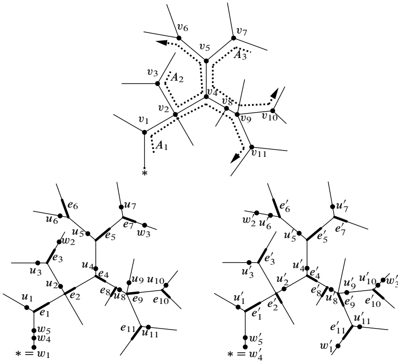
Figure 9: A graph \Gamma (top) and the critical cells \Phi and \Psi in UD^{27}(\Gamma) (bottom left and right)
