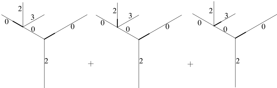
Figure 8: The sum \sum_{i=1}^{d(v)-1} \Theta_{C,v,t,i} with C as in Figure 6
