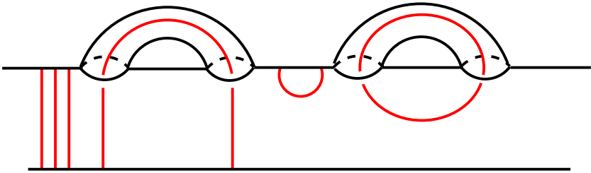
Figure 4: A vp -compressionbody (C, T) . From left to right we have three vertical arcs, one ghost arc, one bridge arc, and one core loop in T .
