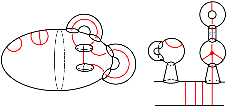
Figure 3: On the left is an example of a vp -compressionbody (C, T) with \partial_-C the union of spheres. On the right is an example of a vp -compressionbody (C, T) with \partial_-C the union of two connected surfaces, one of which is a sphere twice-punctured by T .
