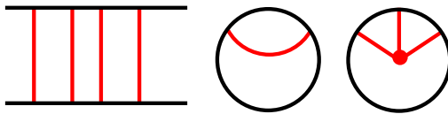
Figure 2: On the left is a trivial product compressionbody; in the center is a trivial ball compressionbody with T an arc; on the right is a trivial ball compressionbody with T a tree having a single interior vertex.
