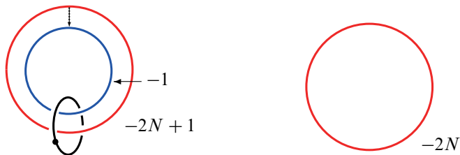
Figure 7: Kirby diagrams of X_j(N) : the dashed arrows indicate how we slide a 2-handle over another one.
