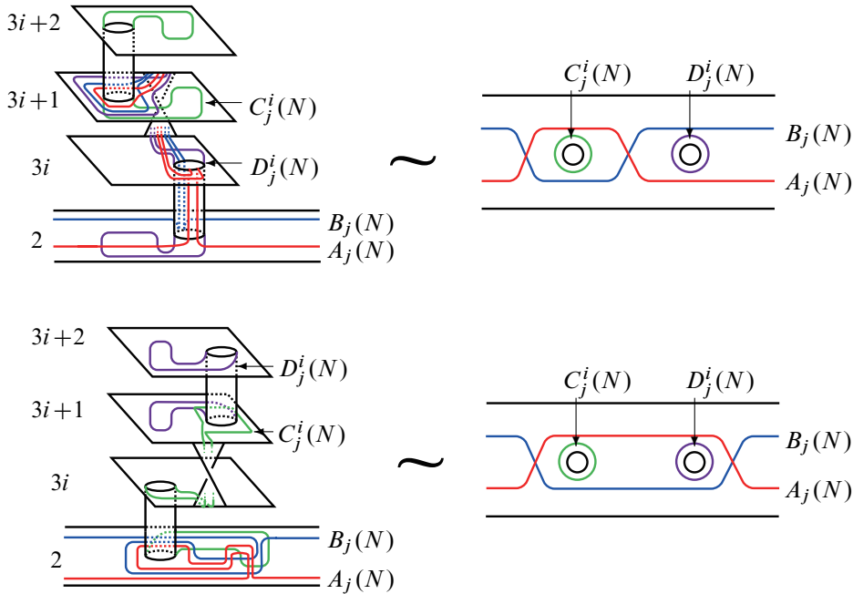
Figure 5: Parts of lifts of arcs a(N) , b(N) , c^i(N) , d^i(N) with respect to q_j(N) . Top: sheets labeled 2, 3i, 3i + 1, 3i + 2 for i = 1, \dots, j - 1 . Bottom: sheets labeled 2, 3i, 3i + 1, 3i + 2 for i = j, \dots, N - 1 .
