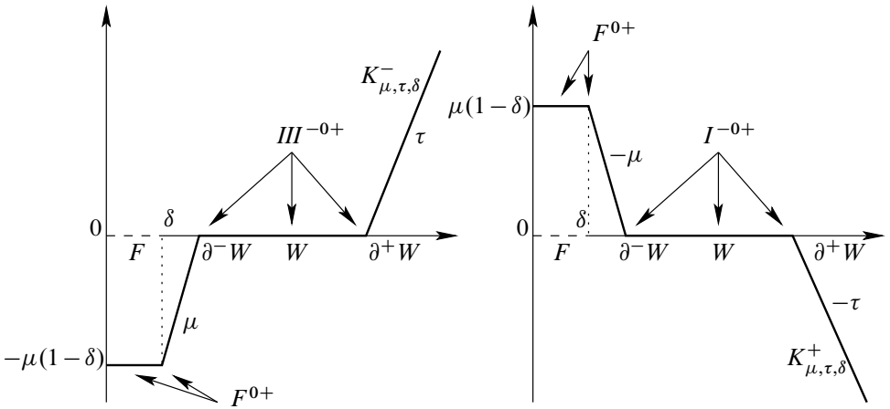
Figure 17: Hamiltonians K^\pm for the definition of \text{SH}_*^\heartsuit(W, \partial^\pm W)
