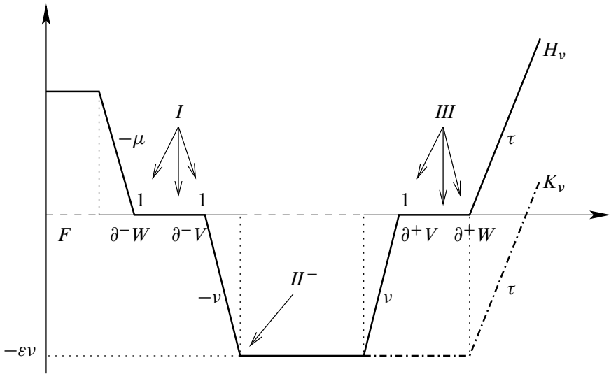
Figure 15: The Hamiltonians H_\nu and K_\nu
