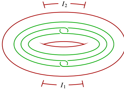
Figure 7: Intervals of S^1 and their clasps
