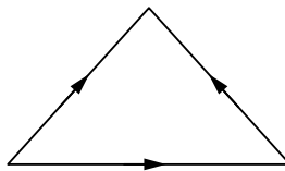
Figure 4: The dunce hat D
