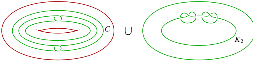
Figure 9: The union of S^1 \times \mathbb{B}^3 with a degree-2 pseudo-2-handle
