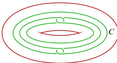
Figure 3: C \subset \partial(S^1 \times \mathbb{B}^3)
