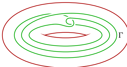
Figure 1: \Gamma \subset \partial(S^1 \times \mathbb{B}^3)
