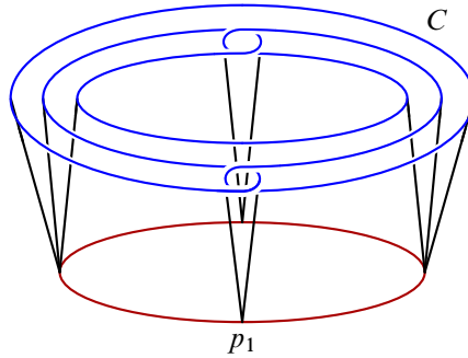
Figure 8: The mapping cylinder of h
