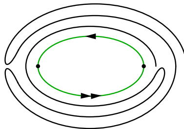
Figure 6: Attaching map for J
