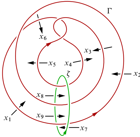
Figure 2: Wirtinger diagram of the Mazur link
