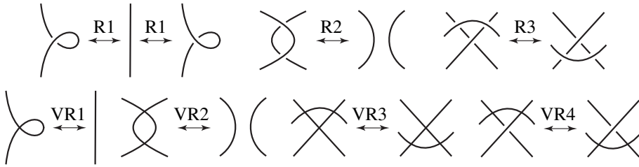
Figure 1: Classical and virtual Reidemeister moves
