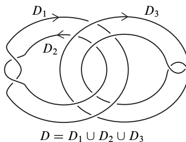
Figure 13: An ordered oriented 3–component classical link diagram with vanishing Alexander polynomial
