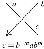
Figure 5: A relation of the generalized link group G_m(D)
