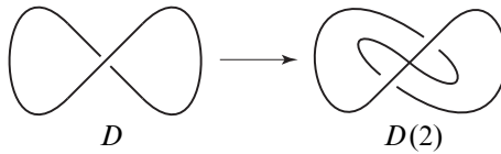
Figure 4: The diagram D(2) , obtained from D by the multiplexing of the crossing, is not virtually isotopic to the trivial knot diagram.
