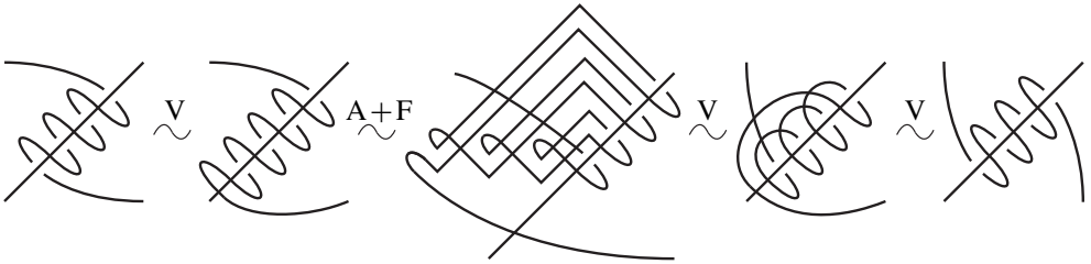
Figure 10: Proof for move C^+
