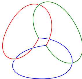
Figure 1: Kinoshita’s knotted theta graph
