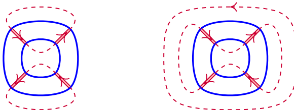
Figure 6: Two completions of the same web. The surrounding dashed circle in the right picture is required by the condition that the unbounded region is painted white.
