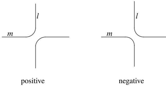
Figure 11: Positive and negative resolutions.
