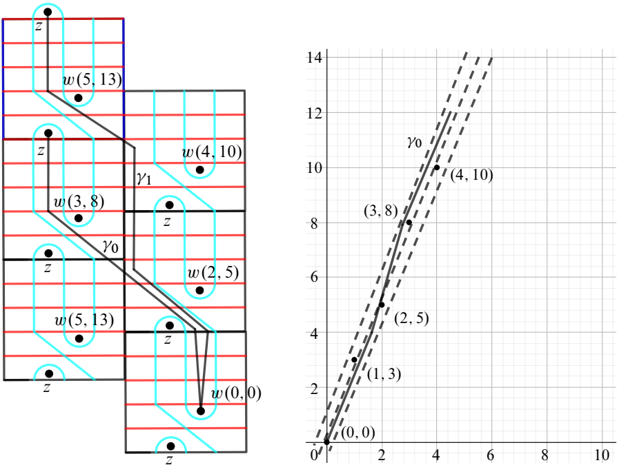
Figure 15: Arcs \gamma_i for C(5, 3, 2, 3, 1) (left) and \gamma_0 for C(5, 3, 2, 3, 1) in \mathbb{R}^2 (right).
