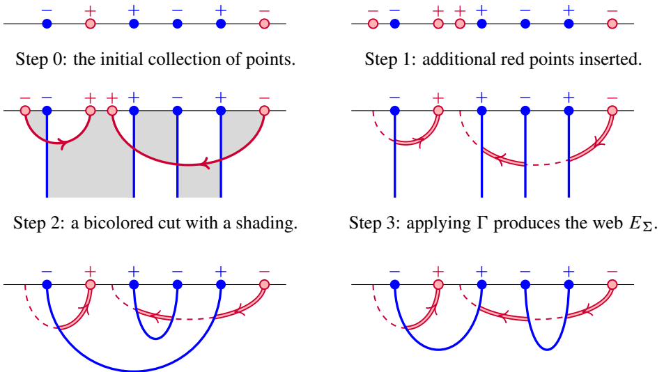
Step 4: connect bottom endpoints in all possible ways to obtain a web basis.
