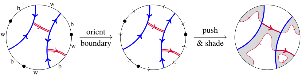
Figure 3: The construction of a shading from a planar web that extends a given shading of its boundary. The boundary of the disk is oriented in the middle picture, whereas the curves U_i^! are identified and pushed inwards the corresponding regions in the third picture.
