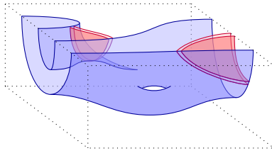
Figure 10: An element of \mathbf{Foam}(a, \omega, b) is a foam in a cube, bounded by the webs \omega, a , and b at the top and opposite vertical facets of the cube respectively.
