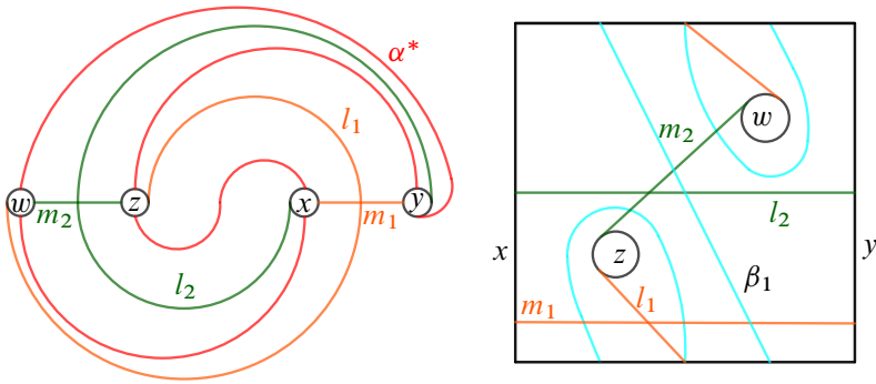
Figure 9: Heegaard diagrams of E(\mathcal{L}(3, 1)) , where \beta_1 is omitted in the left figure and \alpha^* is omitted in the right figure.
