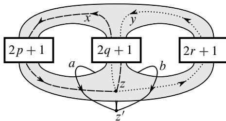
Figure 2: The Seifert surface S of P(2p + 1, 2q + 1, 2r + 1) .
