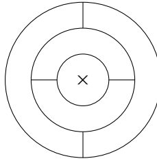
Figure 10: The simplest nonreducible web in the punctured plane.
