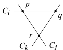
Figure 7: Configuration for C_i, C_j and C_k .
