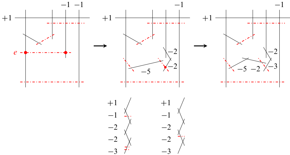
Figure 21: Top: embedding of L_1 in W_1 . Bottom: two curve configurations for Y_L .
