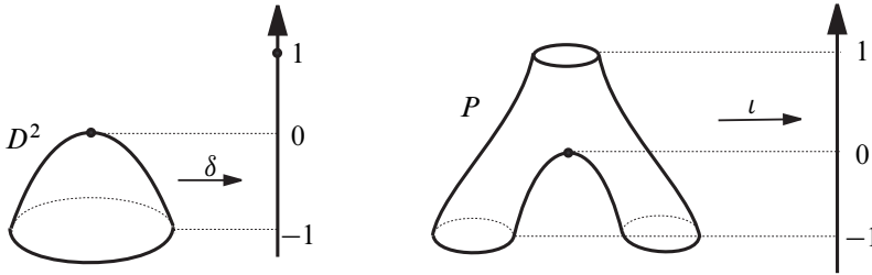
Figure 2: Morse functions \delta and \iota .
