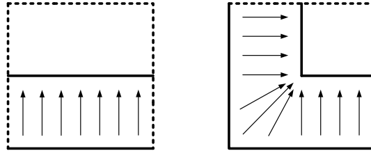
Figure 2: Isotopy from C_k^n(-1) to C_k^n(0) .
