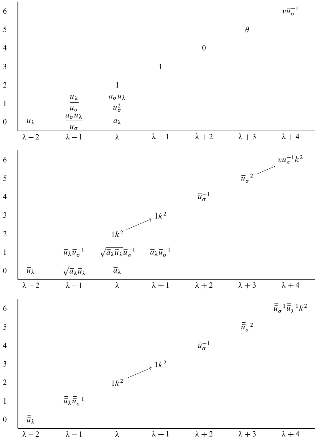
Figure 3: Top: E_1^{\lambda+*,s}(C_4/C_4) , * \in \mathbb{Z} . Center: E_1^{\lambda+*,s}(C_4/C_2) , * \in \mathbb{Z} . Bottom: E_1^{\lambda+*,s}(C_4/e) , * \in \mathbb{Z} .
