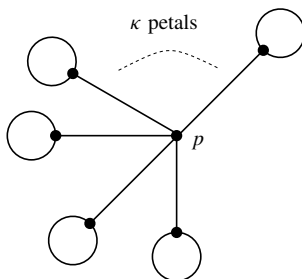
Figure 12. This graph can be lifted to a hyperelliptic curve of genus g if and only if 2g(p) \geq \kappa - 2 . See Example 4.14.
