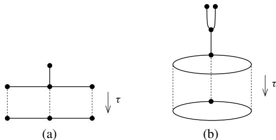
Figure 3. Two tropical modifications.
