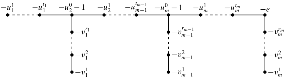
Figure 3. \tilde{\Gamma}_{\tilde{q}, \tilde{p}, m, e} .
