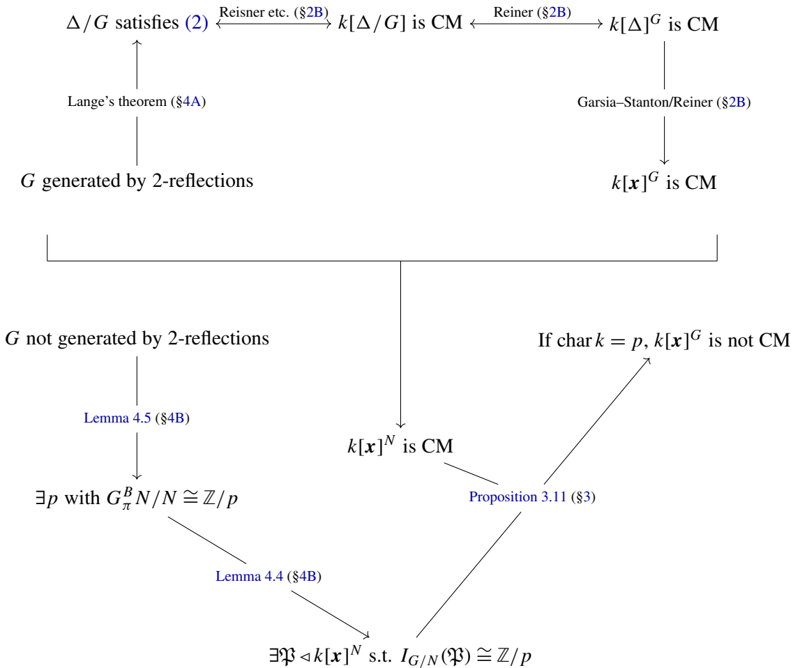
Figure 5. Schematic diagram of the proof of Theorem 1.2 . Arrows are implications, and small print above or interrupting an arrow names a result needed for the implication to go through. The §-references indicate where to look for statements and notation definitions. The top half is the “if” direction ( Proposition 4.1 ). The bottom half is the “only if” direction ( Proposition 4.2 ). The group N is the subgroup of G generated by the 2-reflections, so the “if” direction is required to conclude that k[x]^N is Cohen–Macaulay in the bottom half.
