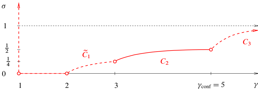
Figure 30. Regularity for global well-posedness on \mathbb{H}^2 .
