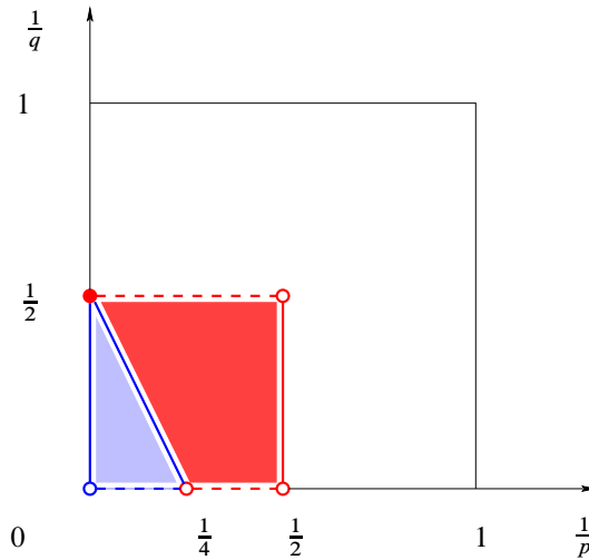
Figure 4. Case n = 2 .
