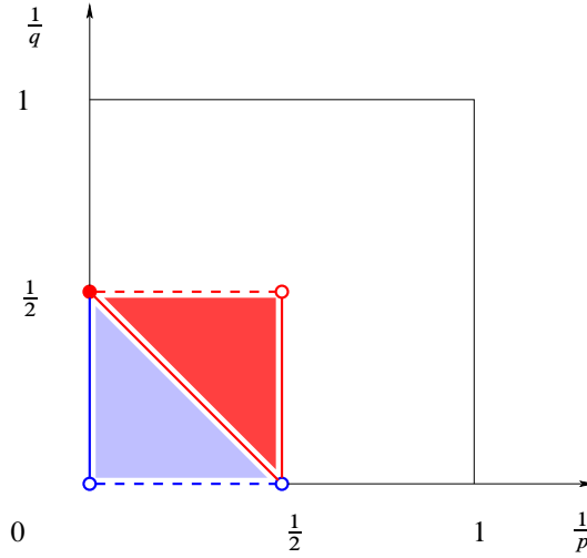
Figure 3. Case n = 3 .
