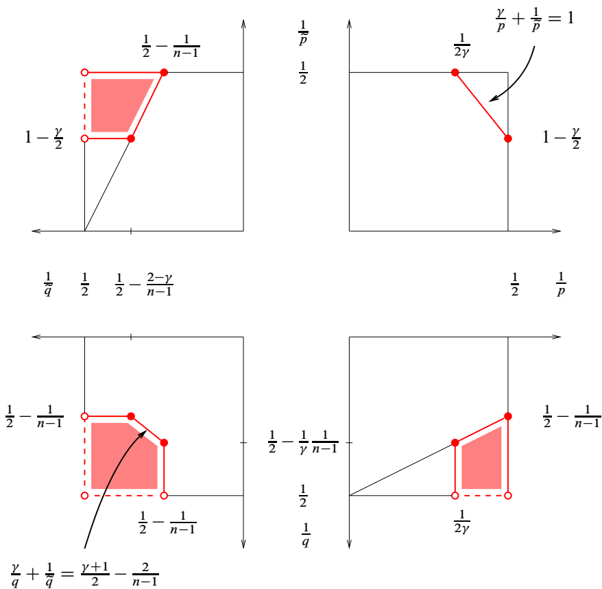
Figure 7. Case \gamma < 2 .
