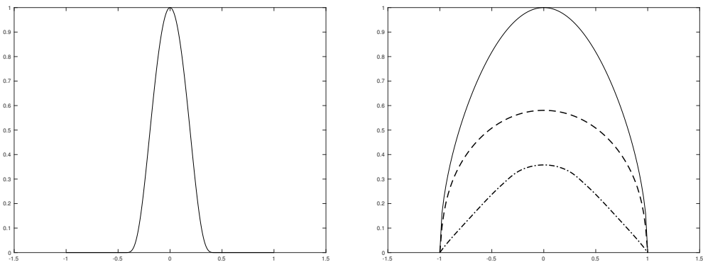
Figure 1. On the left, the initial condition u_0 . On the right, the solid line represents \Phi_1^{1/m} , and the dotted lines represent t^{1/(m-1)}u(t) at t = 1 and t = 5 . The parameters are m = 2 and s = \frac{1}{2} ; hence \sigma = 1 . While u(t) appears to behave as \Phi_1 \propto \text{dist}(\cdot, \partial\Omega) for very short times, already at t = 5 it exhibits the matching boundary behavior predicted by Theorem 5.3.
