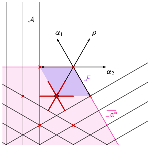
Figure 6. Visualization of the real part of \mathfrak{a}_{\mathbb{C}}^* for G = \text{SL}_3(\mathbb{R}) : The pink region is where Ruelle–Taylor resonances can a priori be located in view of the results of [Bonthonneau et al. 2020] . The red points and lines depict the region where first band resonances can occur: (\mathcal{B} \cap \frac{1}{2} \text{conv}(W\rho) \cup W\rho) - \rho . The purple shaded region illustrates the real parts in which only first band resonances can occur. Further first band resonances might occur inside the exceptional set \mathcal{A} depicted by the black lines.
