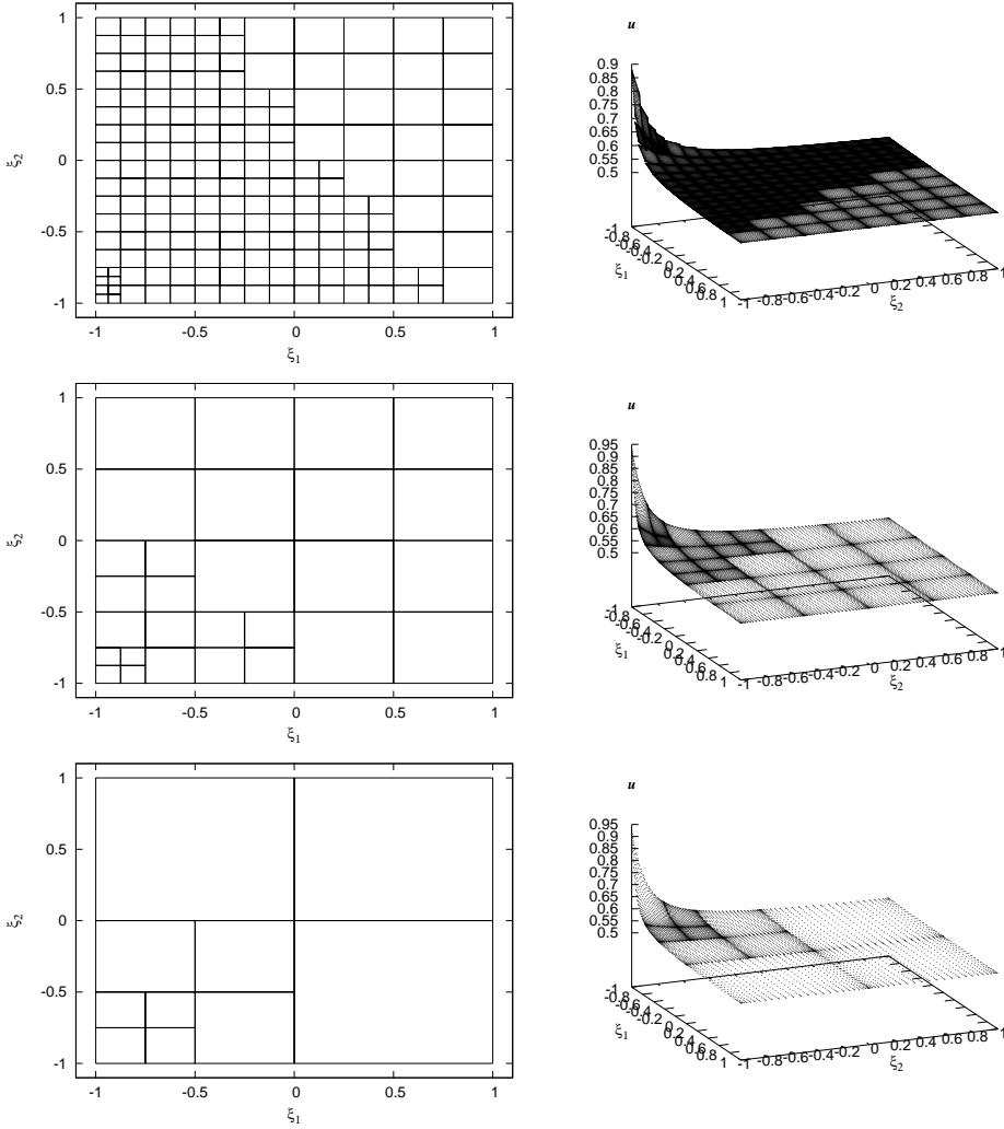
Figure 4. Partition of \Omega_\xi (left) and surface response for U(\xi) at x = 0.1 (right) at the end of the isotropic h_\xi -refinement process using \epsilon = 5.10^{-5} . Plots correspond to q = 1, 3 and 5 from top to bottom.
