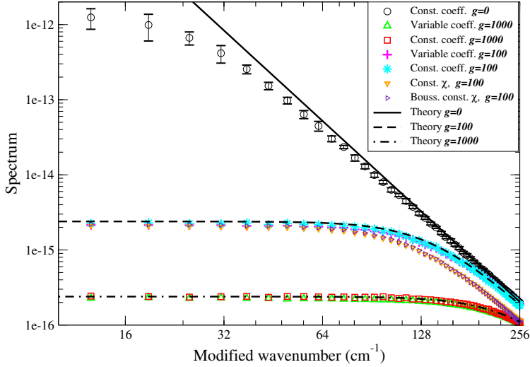
Figure 2. Comparison between the simple theory (A-7) (lines) and numerical results (symbols). Results are shown for standard gravity g \approx 10^3 cm/s 2 (the cutoff wavenumber k_g \approx 246 cm -1 ) for the complete variable-coefficient variable-density low Mach model (green upward triangles) and the constant-coefficient constant-density approximation (red squares). Also shown are results for a weaker gravity, g \approx 10^2 cm/s 2 (the cutoff wavenumber k_g \approx 138 cm -1 ), for the complete low Mach model (magenta pluses) and the constant-coefficient constant-density approximation (cyan stars). For comparison, results for g \approx 10^2 cm/s 2 with variable viscosity \eta(c) but constant diffusion coefficient \chi(c) = \chi_0 are also shown, for variable density (orange downward triangles) and the constant-density (Boussinesq) approximation (indigo right-facing triangles). Finally, results for no gravity are shown in the constant-coefficient approximation (black circles).
