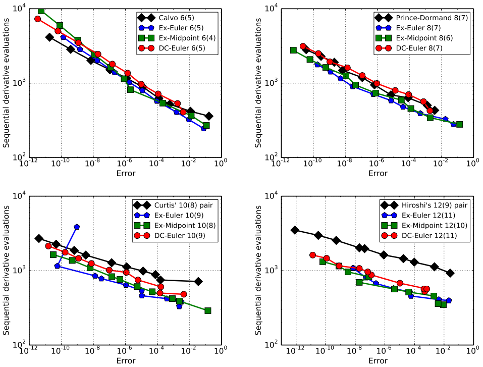
Figure 11. Efficiency for the problem B1 (Section 5.3.2) based on sequential derivative evaluations. Top row: 6th-order methods (left); 8th-order methods (right). Bottom row: 10th-order methods (left); 12th-order methods (right).
