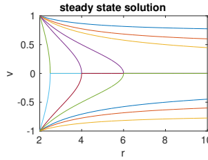
Figure 1. Burgers: steady state solutions.
