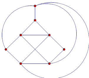
Figure 3. An immersion of P_8 - e_{3,3} with only one crossing.
