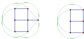
Figure 2. Vertex classes of K_{3,3} - e_{4,6} and the subgraph H .
