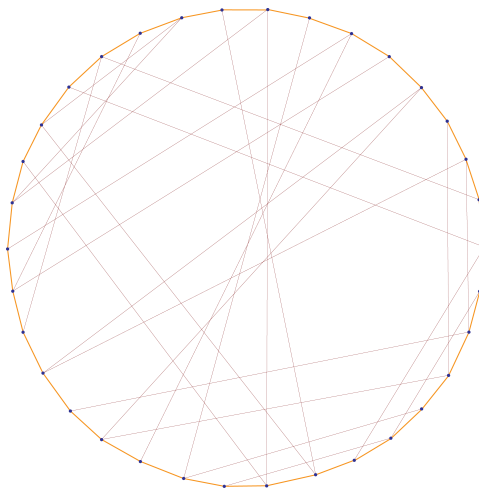
Figure 13. \Phi_3 with Hamiltonian cycle highlighted.
