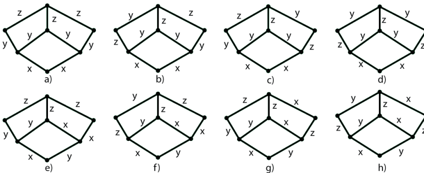
Figure 6. Possible labeled subquivers.
