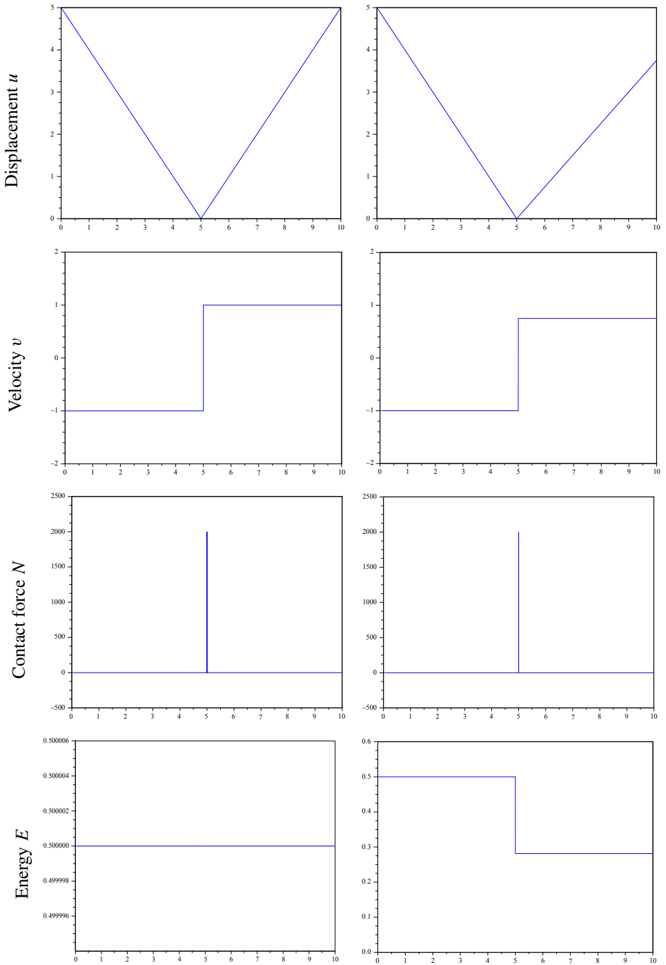
Figure 3. Numerical results without considering the coefficient of restitution (left) and with \text{COR} = 0.75 (right).
